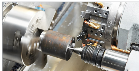
BAR TURNING
